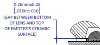
DETAIL B SCALE 3 : 1
