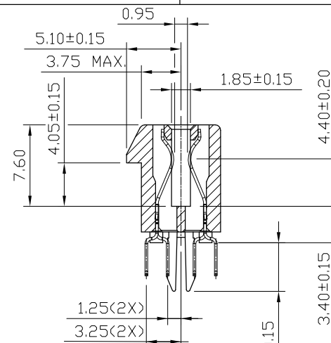
SECTION P-P
