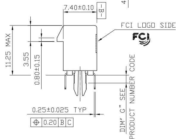
SECTION P-P
