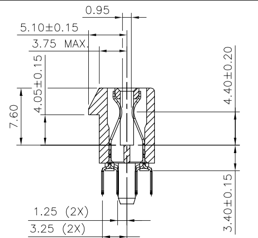
SECTION P-P
