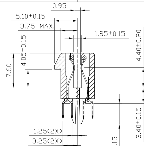
SECTION P-P
