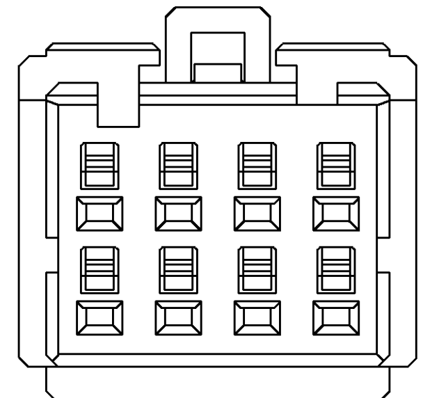
1-1939028-4 8POS:NATURAL,X-KEY 3-1939028-4 8POS:YELLOW,X-KEY
