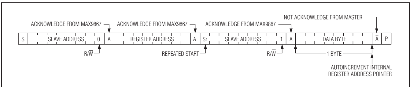
Figure 14. Reading 1 Byte of Data from the MAX9867
