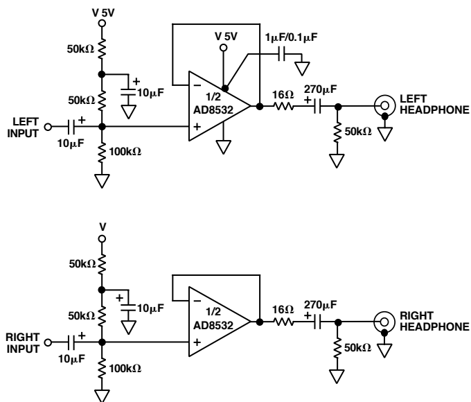
Figure 40. A Single-Supply, Stereo Headphone Driver
