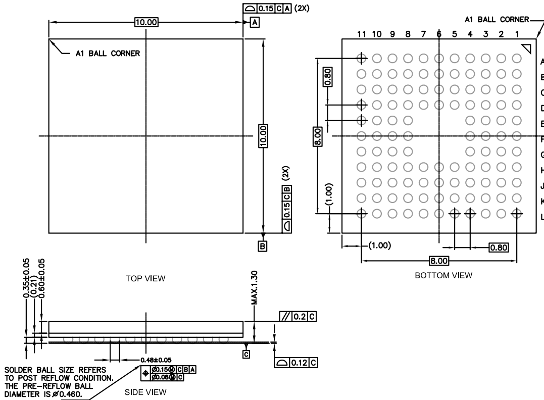
Figure 4.2. BGA112
