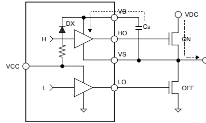
Figure 8. Discharging Period
