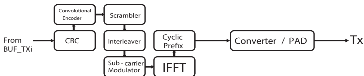
Figure 9-2. Transmission Branch
