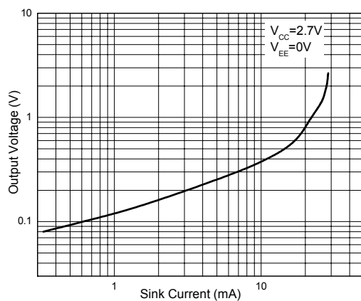
Figure 14. Output Voltage vs. Output Sink Current
