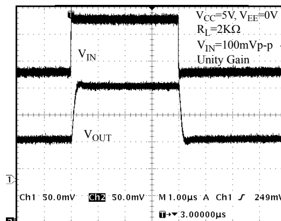
Figure 21. Non-Inverting Input Small Signal Pulse Response
