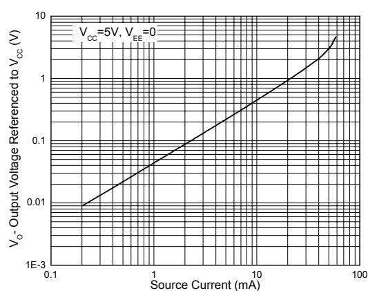
Figure 11. Output Voltage vs. Output Source Current
