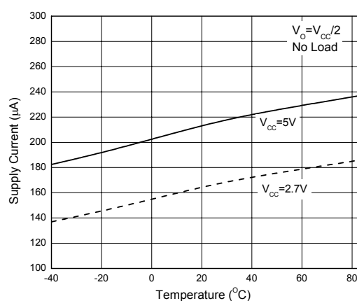
Figure 5. Supply Current vs. Temperature
