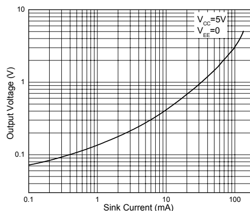
Figure 13. Output Voltage vs. Output Sink Current
