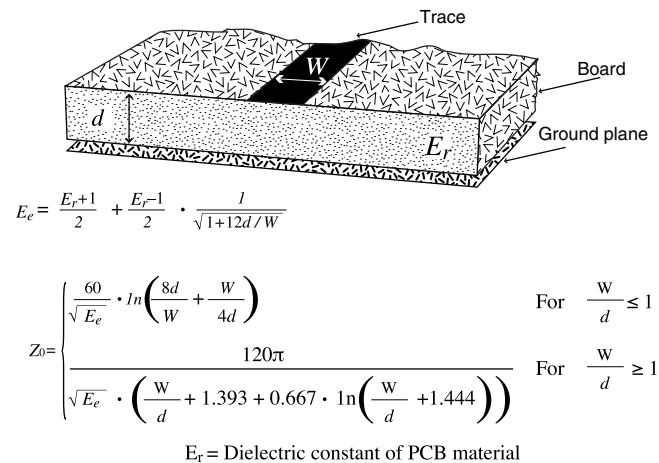
Figure 51: Microstrip Formulas
