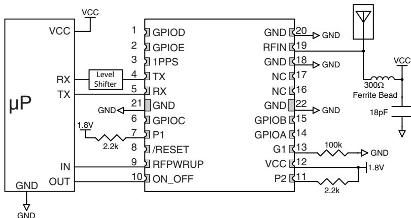
Figure 47: Circuit Using the F4 Series Module with a an Active Antenna
