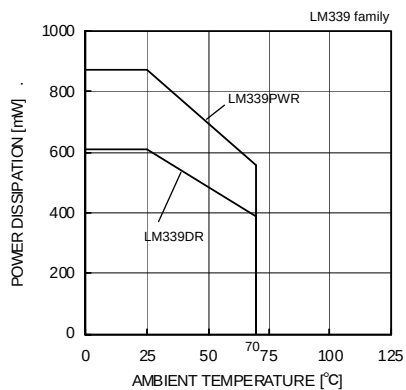
Fig. 21 Derating Curve
