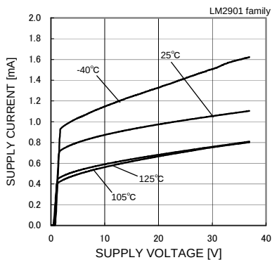
Supply Current – Supply Voltage
