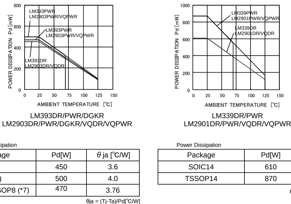
Fig.91 Derating Curves
