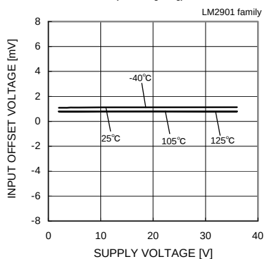
Input Offset Voltage – Supply Voltage
