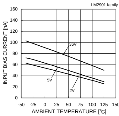
Input Bias Current – Ambient Temperature
