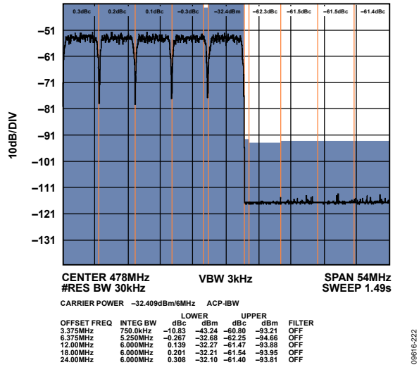
Figure 149. 64-Carrier Low Band Narrow-Band ACLR
