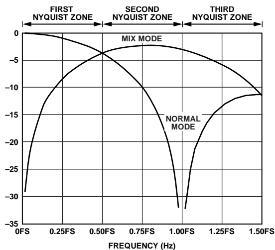
Figure 172. Sinc Roll-Off for Each Analog Operating Mode
