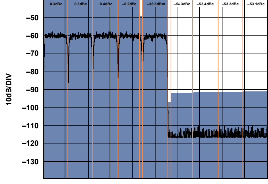
Figure 76. 64-Carrier High Band Narrow-Band ACLR
