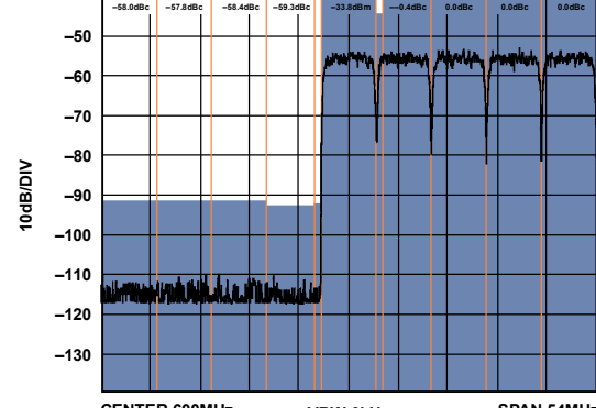
Figure 75. 64-Carrier Low Band Narrow-Band ACLR
