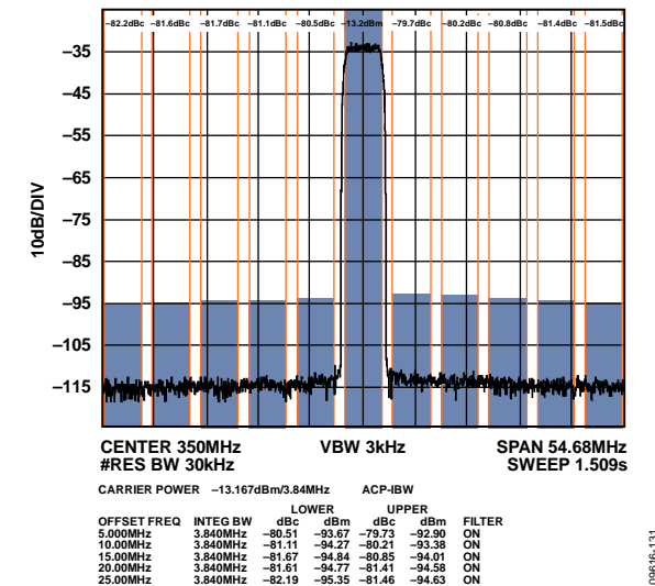
Figure 31. Single-Carrier WCDMA at 350 MHz, f_{DAC} = 2457.6 MSPS
