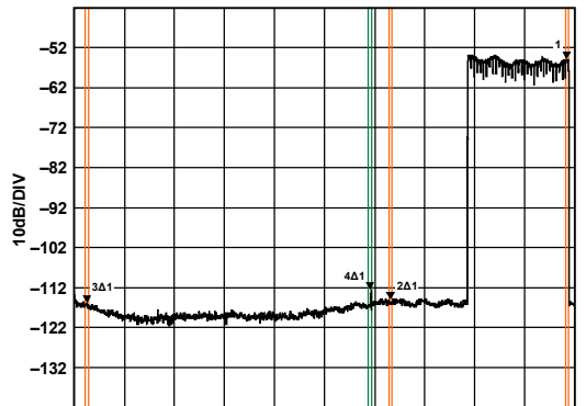
Figure 141. Mid Band Wideband ACLR
