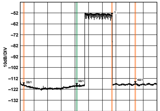
Figure 140. Low Band Wideband ACLR
