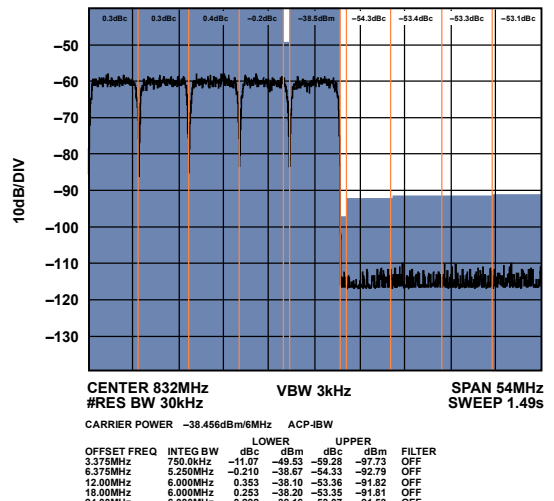
Figure 77. 128-Carrier Narrow-Band ACLR
