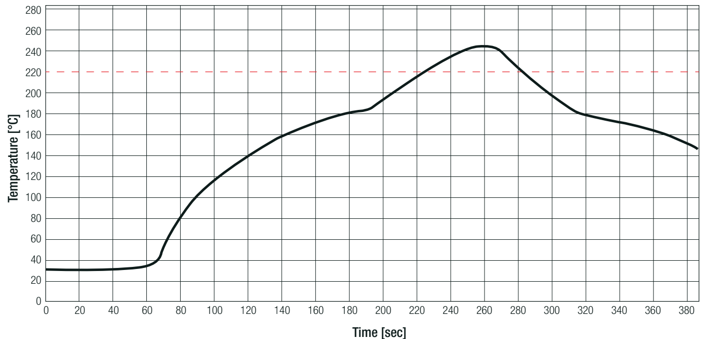
Lead-free Recommended Solder Profile according to JEDEC STD-020D-01
