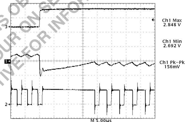
Figure 9. CS5151 Demonstration Board Response to a 0.5 to 13 A Load Pulse (Output Set for 2.8 V)
