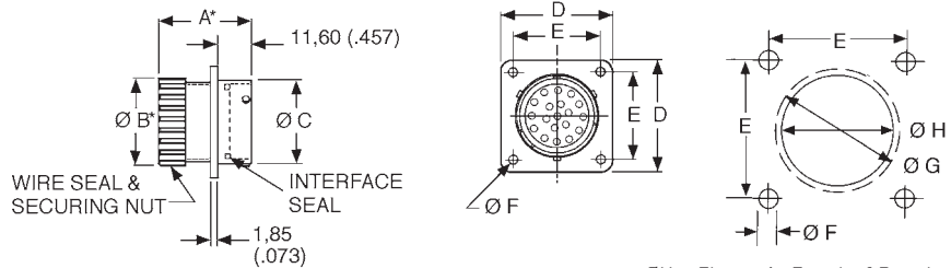
Panel Cutout
