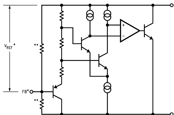
Block Diagram
