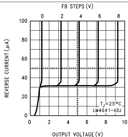
Figure 12. Reverse Characteristics
