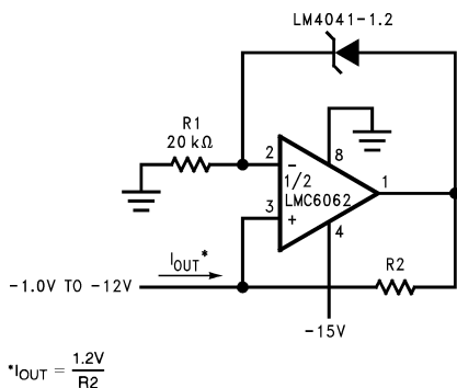
Figure 24. Precision 1-μA to 1-mA Current Sink
