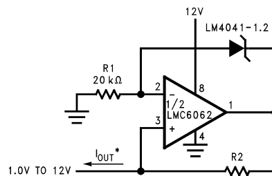
Figure 25. Precision 1-μA to 1-mA Current Sources
