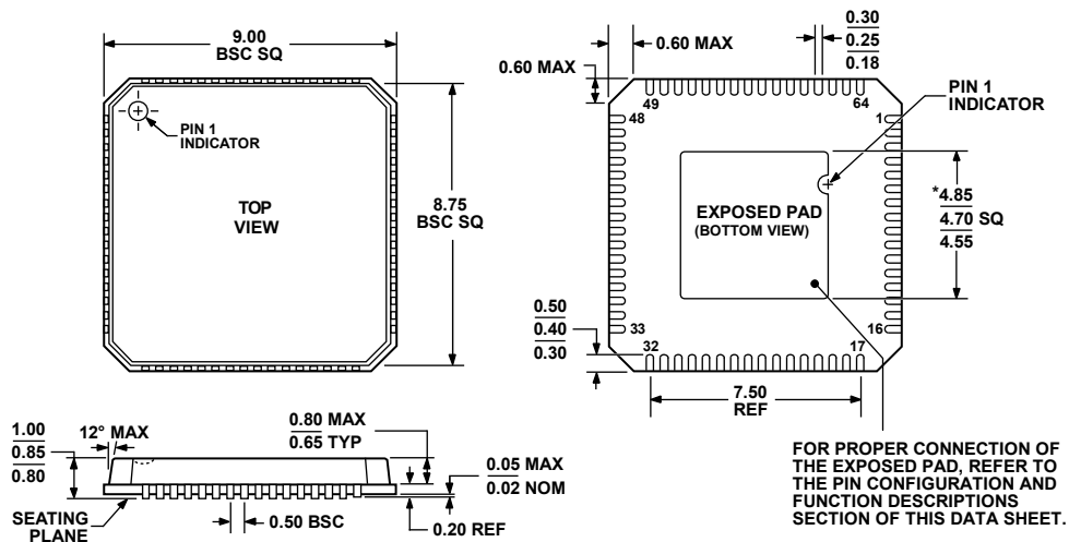
Figure 125. 64-Lead Lead Frame Chip Scale Package (LFCSP_VQ) 9 mm x 9 mm Body, Very Thin Quad (CP-64-1) Dimensions shown in millimeters
