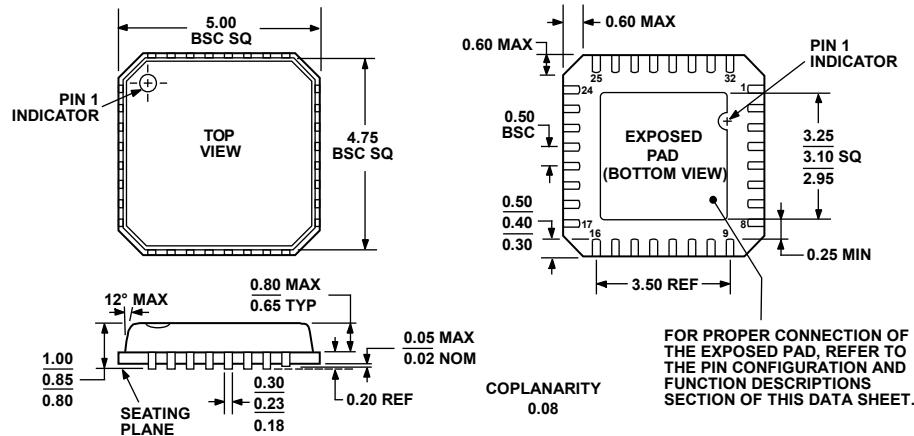
Figure 124. 32-Lead Lead Frame Chip Scale Package (LFCSP_VQ) 5 mm x 5 mm Body, Very Thin Quad (CP-32-2) Dimensions shown in millimeters
