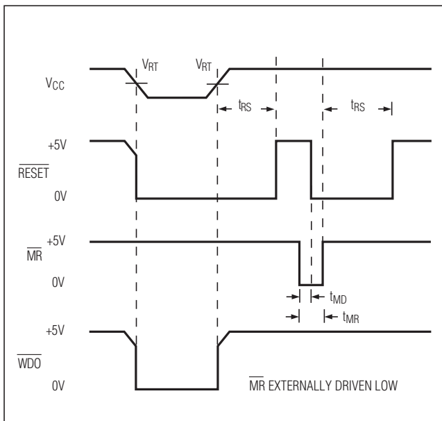
Figure 4. MAX705/MAX706 \overline{\text{RESET}} , \overline{\text{MR}} , and \overline{\text{WDO}} Timing with WDI Three-Stated. The MAX707/MAX708/MAX813L \text{RESET} output is the inverse of \overline{\text{RESET}} shown.
