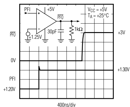
POWER-FAIL COMPARATOR DE-ASSERTION RESPONSE TIME
