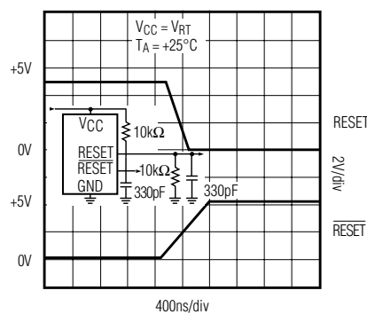
MAX707 RESET, RESET DE-ASSERTION
