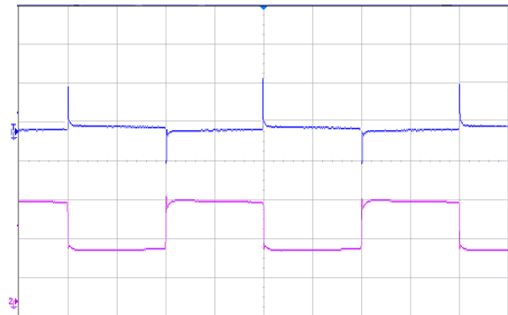
Figure 5 Dynamic response for 25% load step (25% ~ 50% ~ 25%) and 1A/ \mu\text{s} slew rate (2ms/div), see Figure 11 for test configuration; CH1-output voltage (100mV/div); CH2-output current (10A/div)
