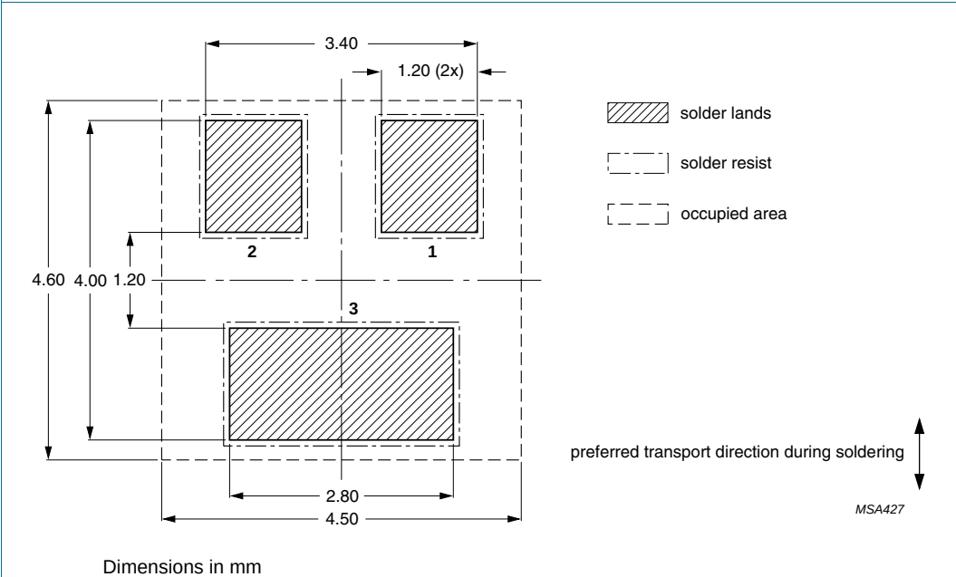
Fig 18. Wave soldering footprint SOT23 (TO-236AB)
