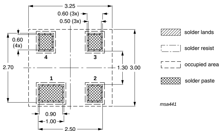
Fig 23. Reflow soldering footprint SOT143B
