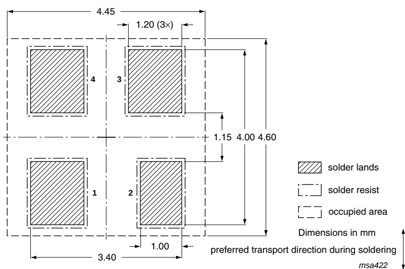
Fig 23. Reflow soldering footprint SOT143B
