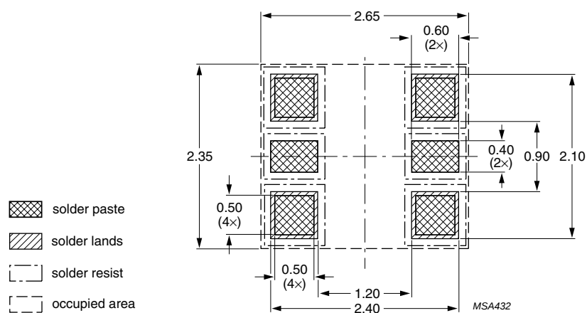
Fig 25. Reflow soldering footprint SOT363 (SC-88)
