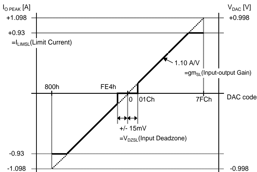
Figure 12. I_{O\text{ PEAK}} Characteristics (When set as R_{SLRNF}=0.56\ \Omega ).
