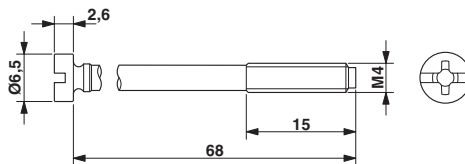
Dimensioned drawing
