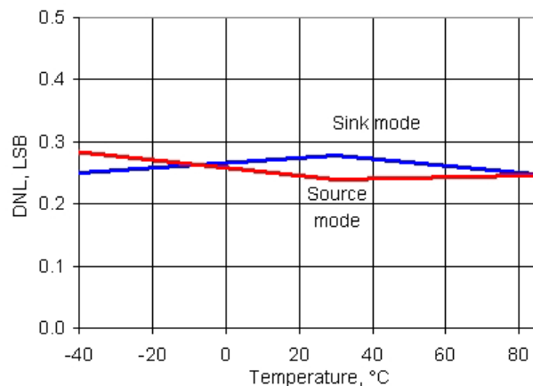
Figure 11-41. IDAC DNL vs Temperature, Range = 255 \mu A, High speed mode
