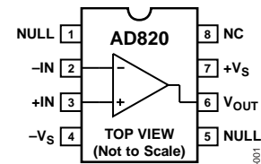
Figure 1. 8-Lead PDIP
