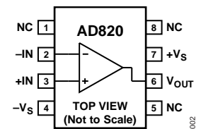
Figure 1. 8-Lead PDIP
