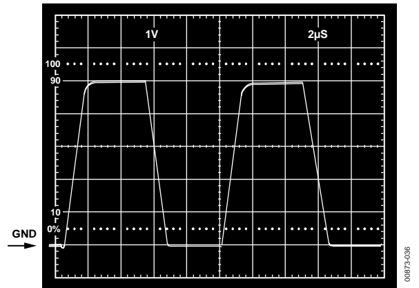
Figure 36. V_S = 5\text{ V}, 0\text{ V} ; Gain-of-2 Inverter Response to 2.5 V Step, Centered -1.25 V Below Ground
