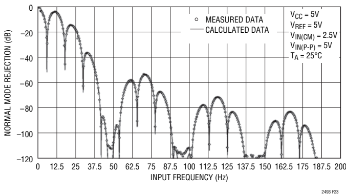
Figure 23. Input Normal Mode Rejection vs Input Frequency with Input Perturbation of 100% (50Hz/60Hz Notch)
