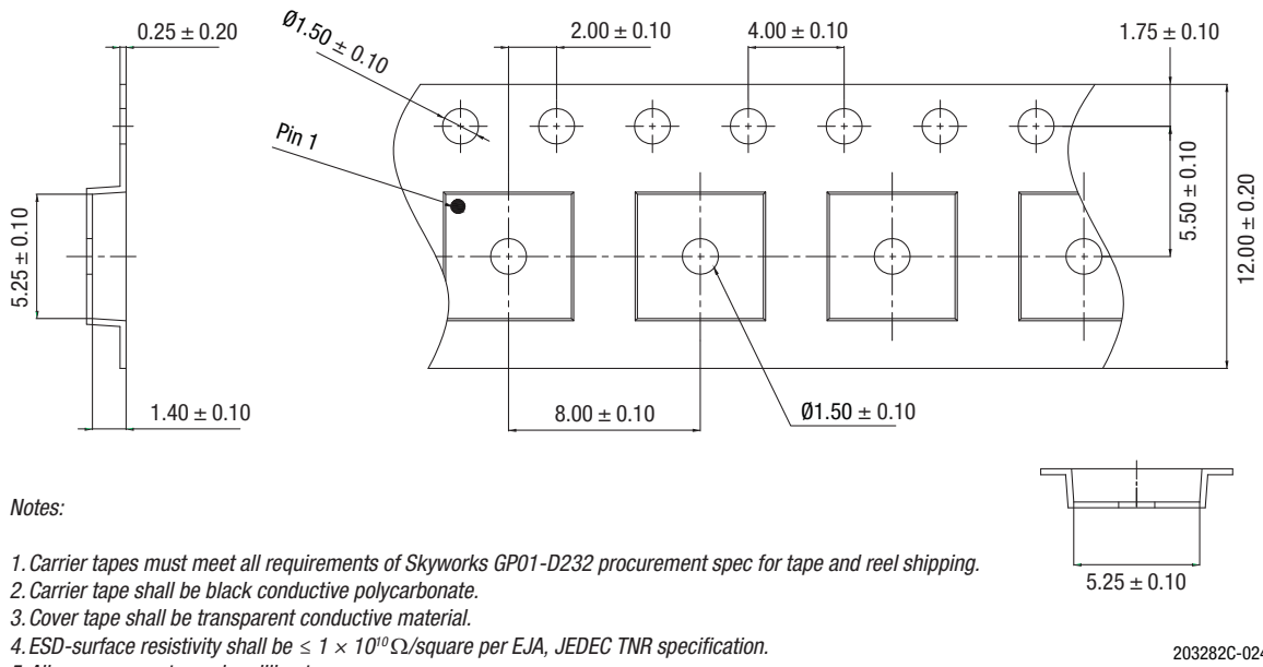
Figure 24. SKY66292-11 Tape and Reel Dimensions
