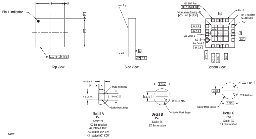
Figure 23. SKY66292-11 Package Dimensions
