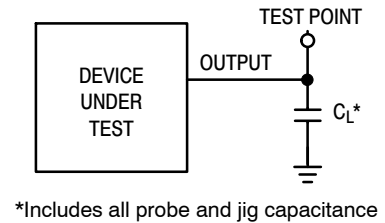
Figure 3. Test Circuit
