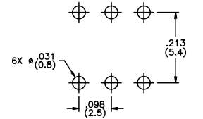
P.C. board layout
