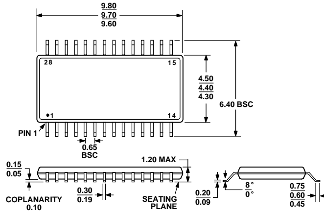
COMPLIANT TO JEDEC STANDARDS MO-153-AE Figure 69. 28-Lead Thin Shrink Small Outline Package [TSSOP] (RU-28) Dimensions shown in millimeters
