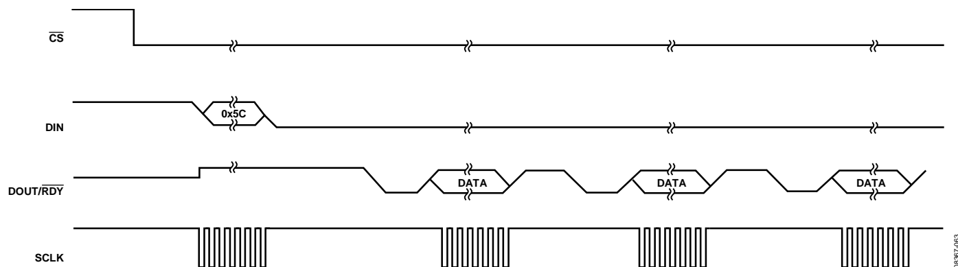
Figure 27. Continuous Read
