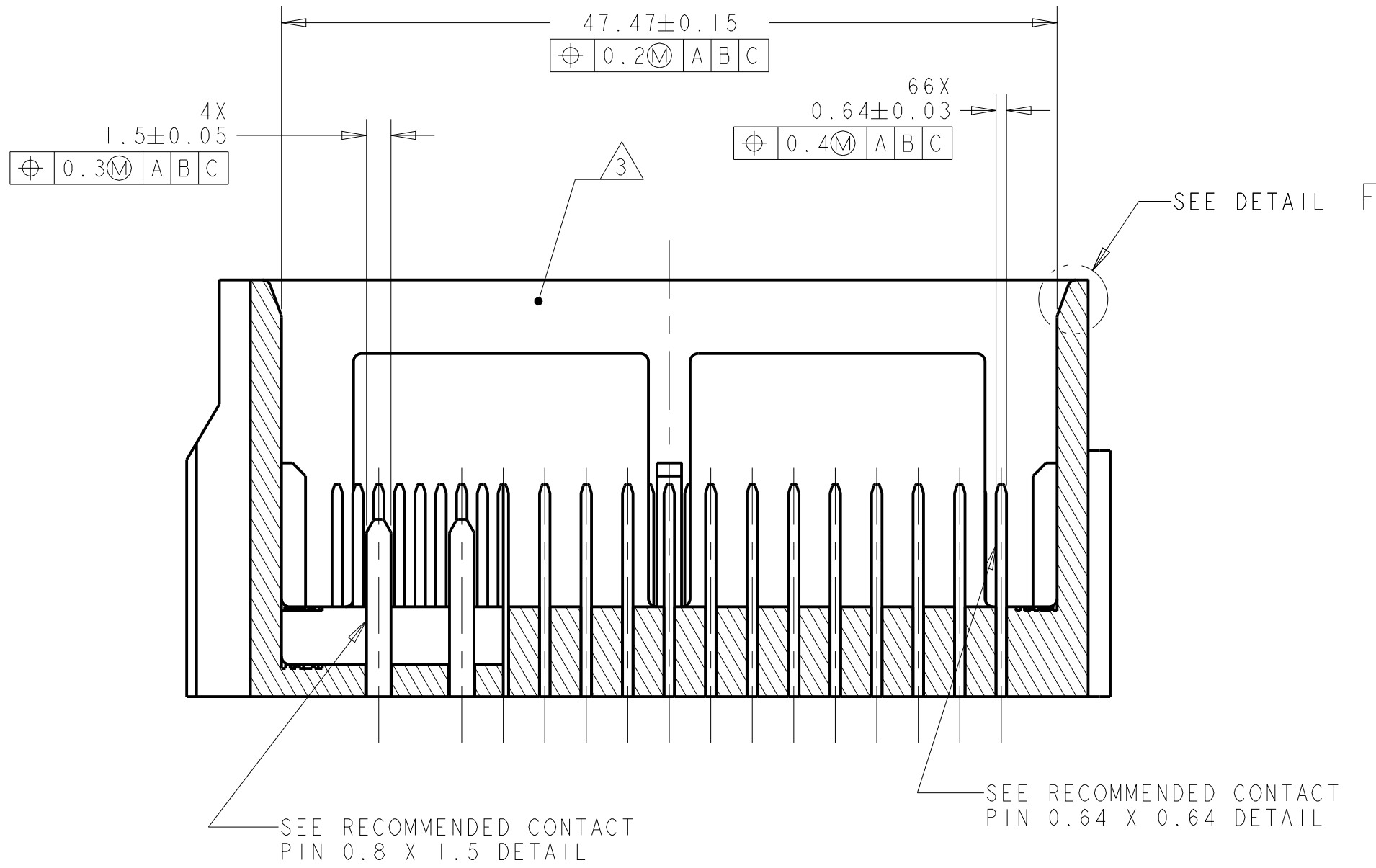
SECTION B-B
