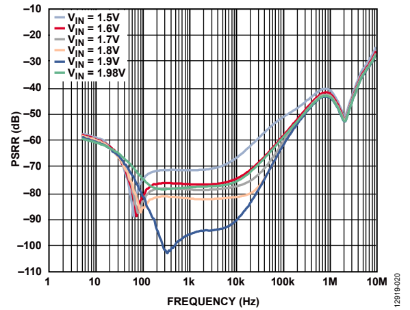
Figure 20. Power Supply Rejection Ratio (PSRR) vs. Frequency for Various V_{IN} , V_{OUT} = 1.3 V, Load Current = 1 A
