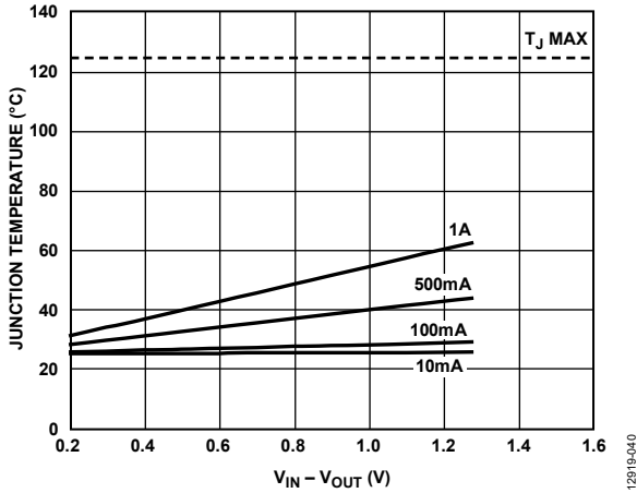
Figure 40. 500 mm 2 of PCB Copper, T B = 25°C
