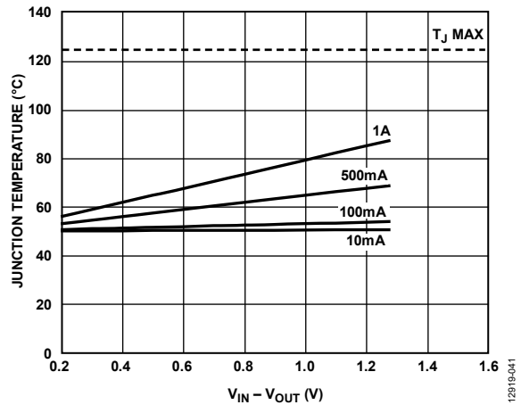
Figure 41. 500 mm 2 of PCB Copper, T B = 50°C
