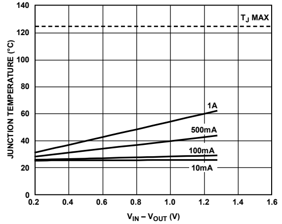
Figure 42. 1000 mm 2 of PCB Copper, T B = 25°C
