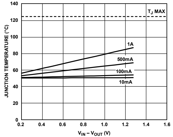
Figure 43. 1000 mm 2 of PCB Copper, T B = 50°C
