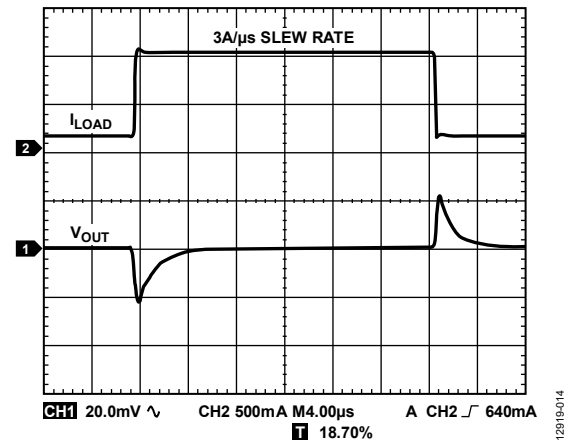
Figure 14. Load Transient Response, C_{OUT} = 10\text{ }\mu\text{F} , V_{IN} = 1.7\text{ V} , V_{OUT} = 1.3\text{ V}
