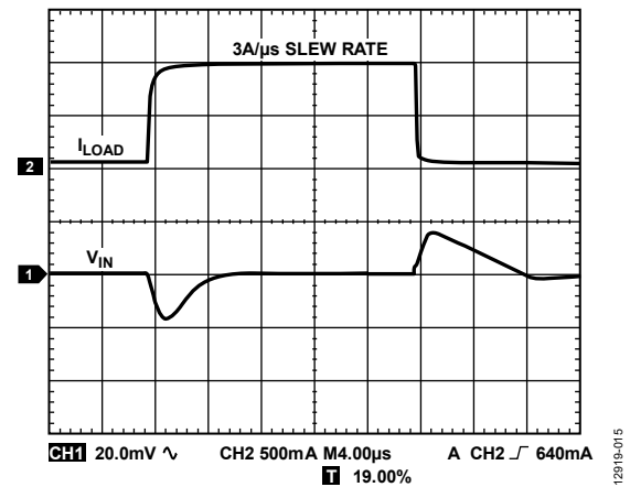
Figure 15. Load Transient Response, C_{OUT} = 47\text{ }\mu\text{F} , V_{IN} = 1.7\text{ V} , V_{OUT} = 1.3\text{ V}
