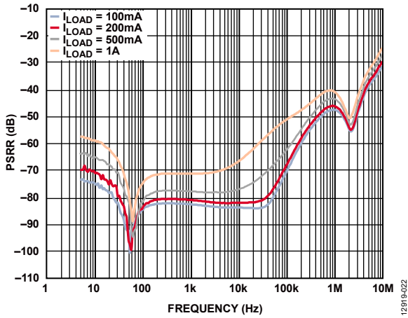
Figure 22. Power Supply Rejection Ratio (PSRR) vs. Frequency for Various Loads, V_{OUT} = 1.3 V , V_{IN} = 1.5 V
