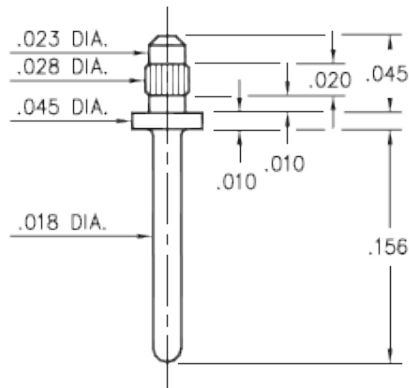
9159-0-00-XX-00-00-03-0 Press-fit in .026 mounting hole
