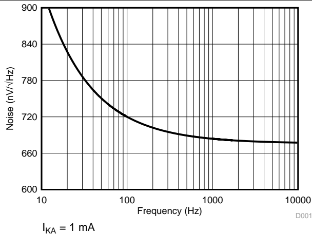
Figure 9. Noise Voltage
