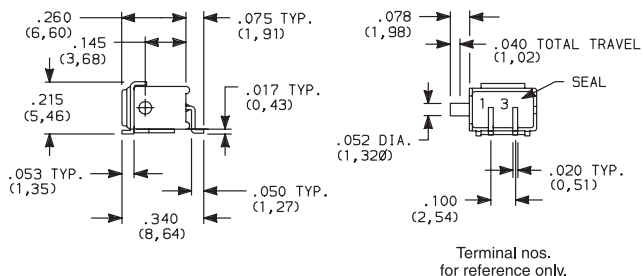
GP11MSA1BE SPST
