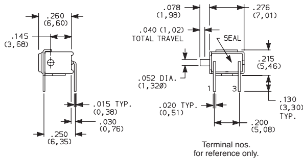
GP11MABE SPST
