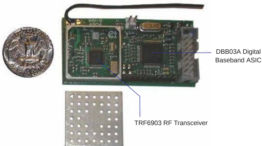
Figure 3–3. Dolphin Low Power Board
