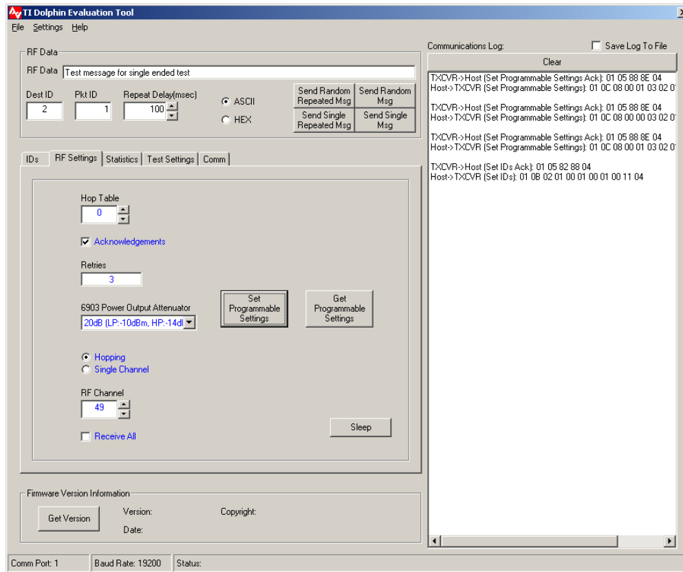
Figure 4–10. ID Setup for Round-Trip Test
