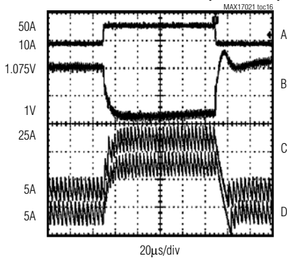
LOAD TRANSIENT RESPONSE (HFM MODE)
