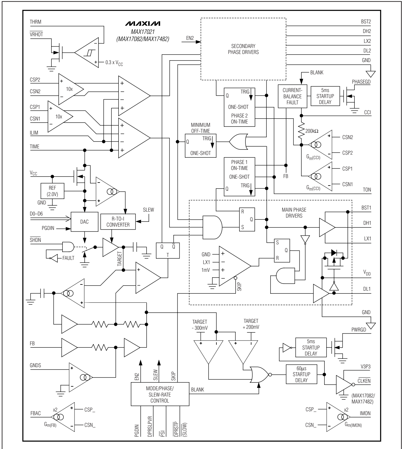
Figure 3. Functional Diagram
