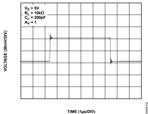
Figure 21. Small Signal Transient Response
