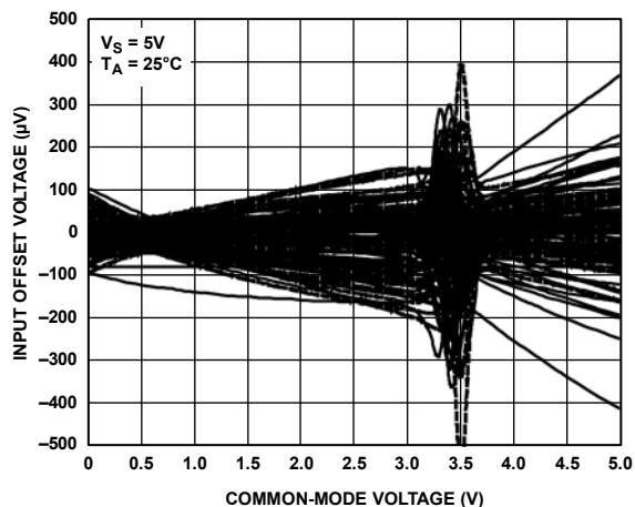
Figure 8. Input Offset Voltage vs. Common-Mode Voltage (200 Units, Five Wafer Lots Including Process Skews)
