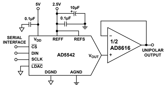
Figure 42. Buffering DAC Output
