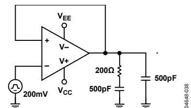
Figure 38. Snubber Network
