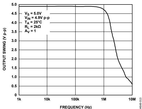
Figure 13. Closed-Loop Output Voltage Swing vs. Frequency
